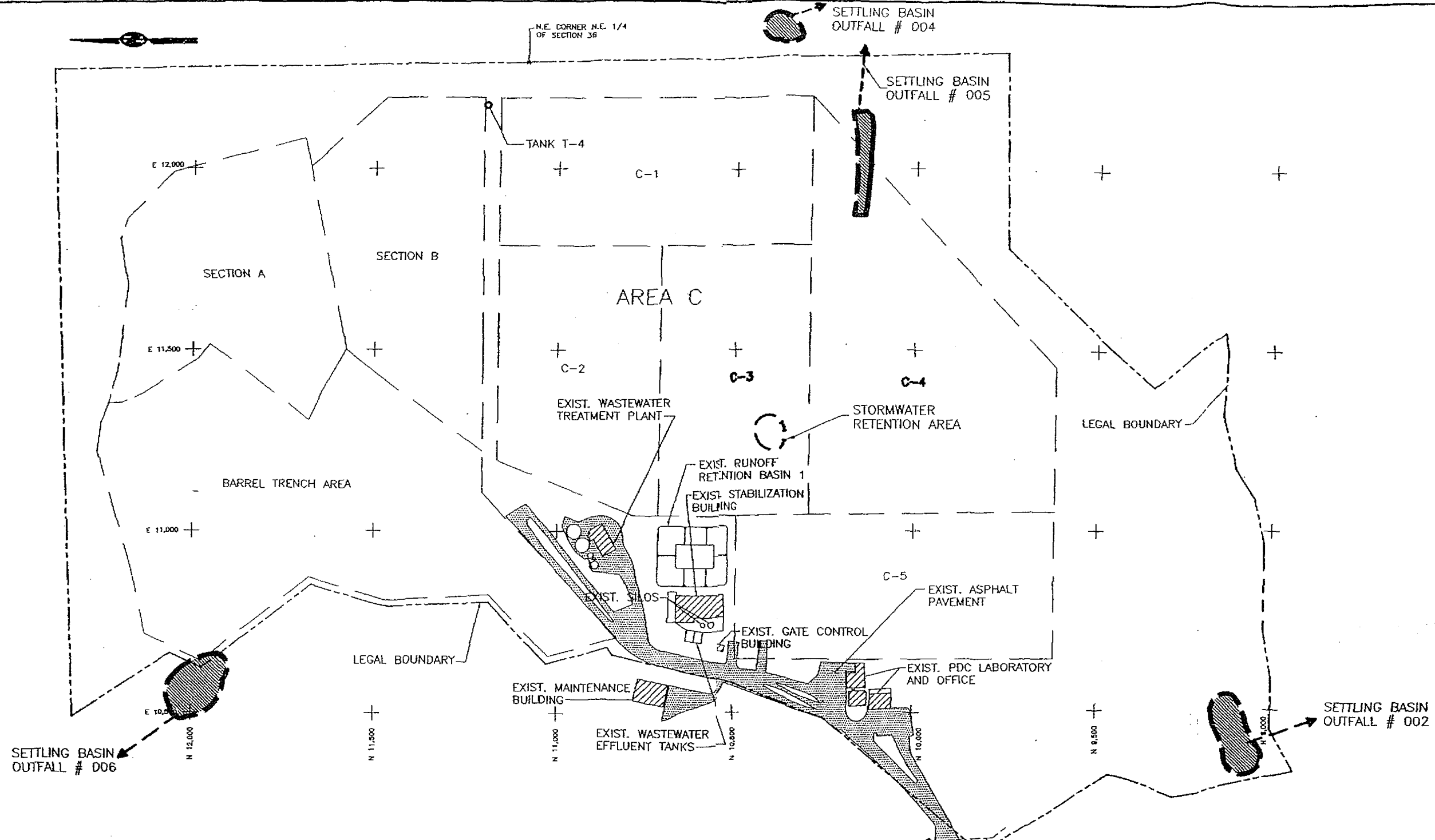
Figure 5 Site Layout PDC RCRA FACILITY STORMWATER PEORIA, ILLINOIS PDC Technical Services, Inc. Project No. 92C-217 PREPARED BY: AUSTIN ENGINEERING CO., INC. PEORIA, ILLINOIS
